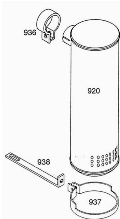
Figure 1 — Replacement Parts Illustration
