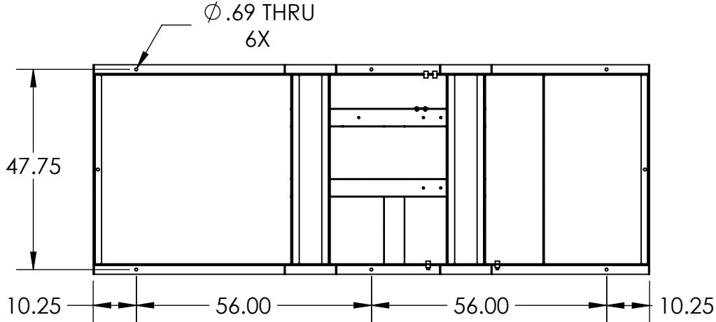
TOP VIEW HOLE PATTERN
